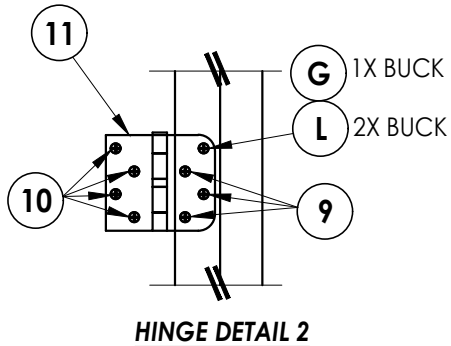
HINGE DETAIL 2
