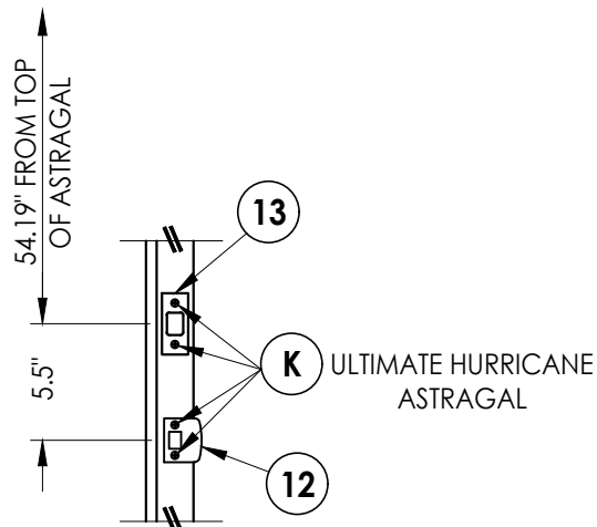
LATCH AND DEADBOLT STRIKE DETAILS
