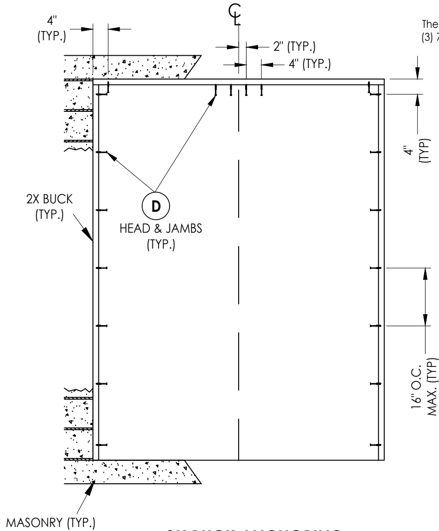
2X BUCK ANCHORING
